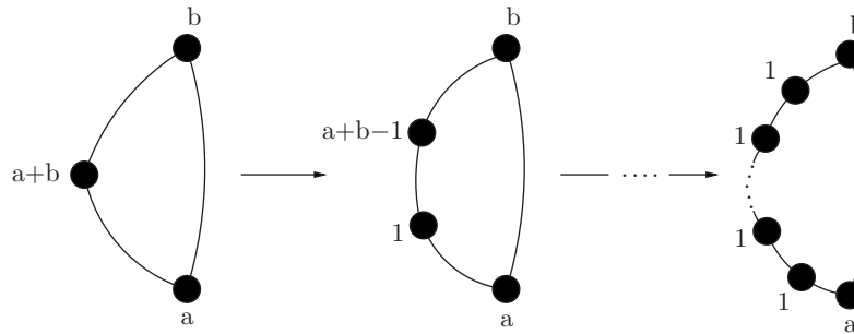
FIGURE 2. Blowing up fixed points of index 2
